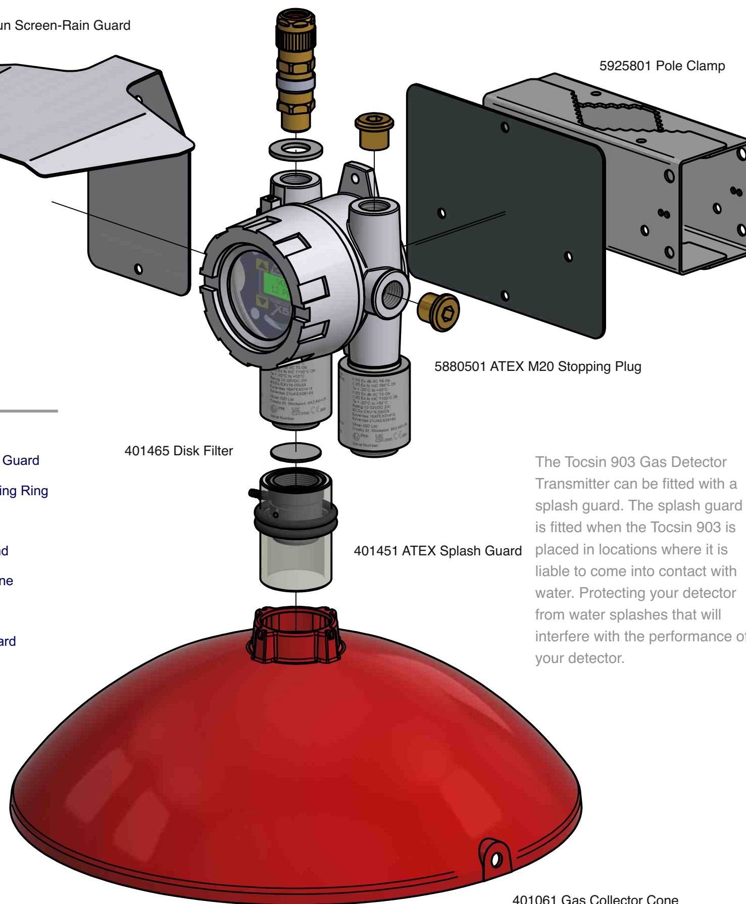
401061 Gas Collector Cone
